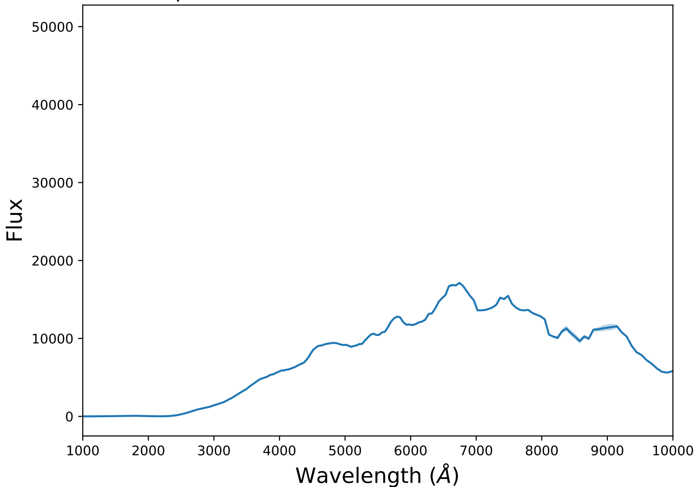
Spectrum 2 for transient SLSN at z=2.08
